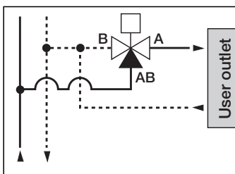
3-way installed on the flow pipe with diverter position and ON/OFF operation
