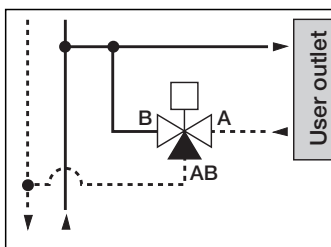
3-way installed on the return pipe with mixer position and ON/OFF operation
